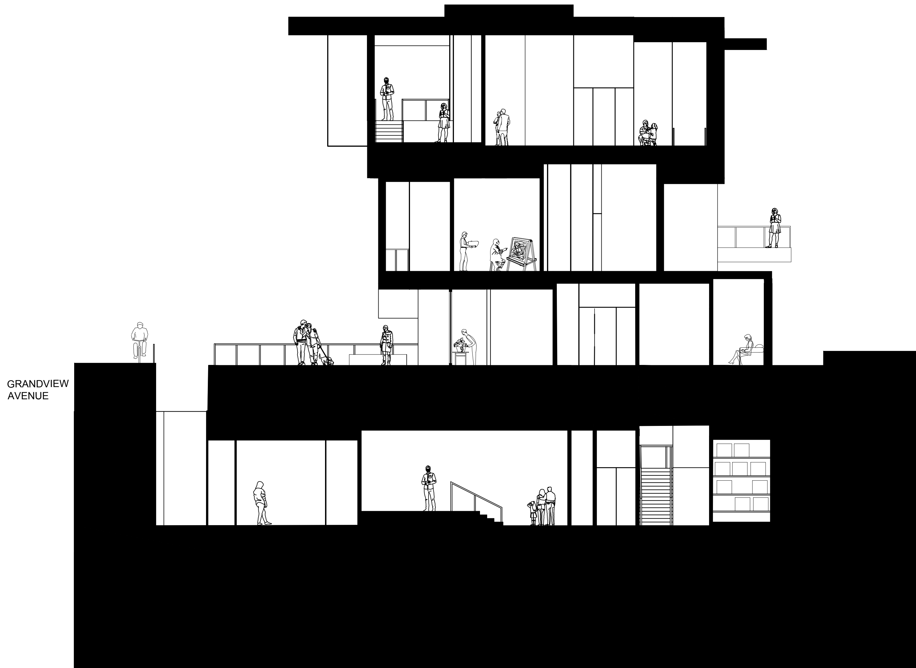
SECTION A-A SCALE = 1'-0" = \frac{1}{8} "
