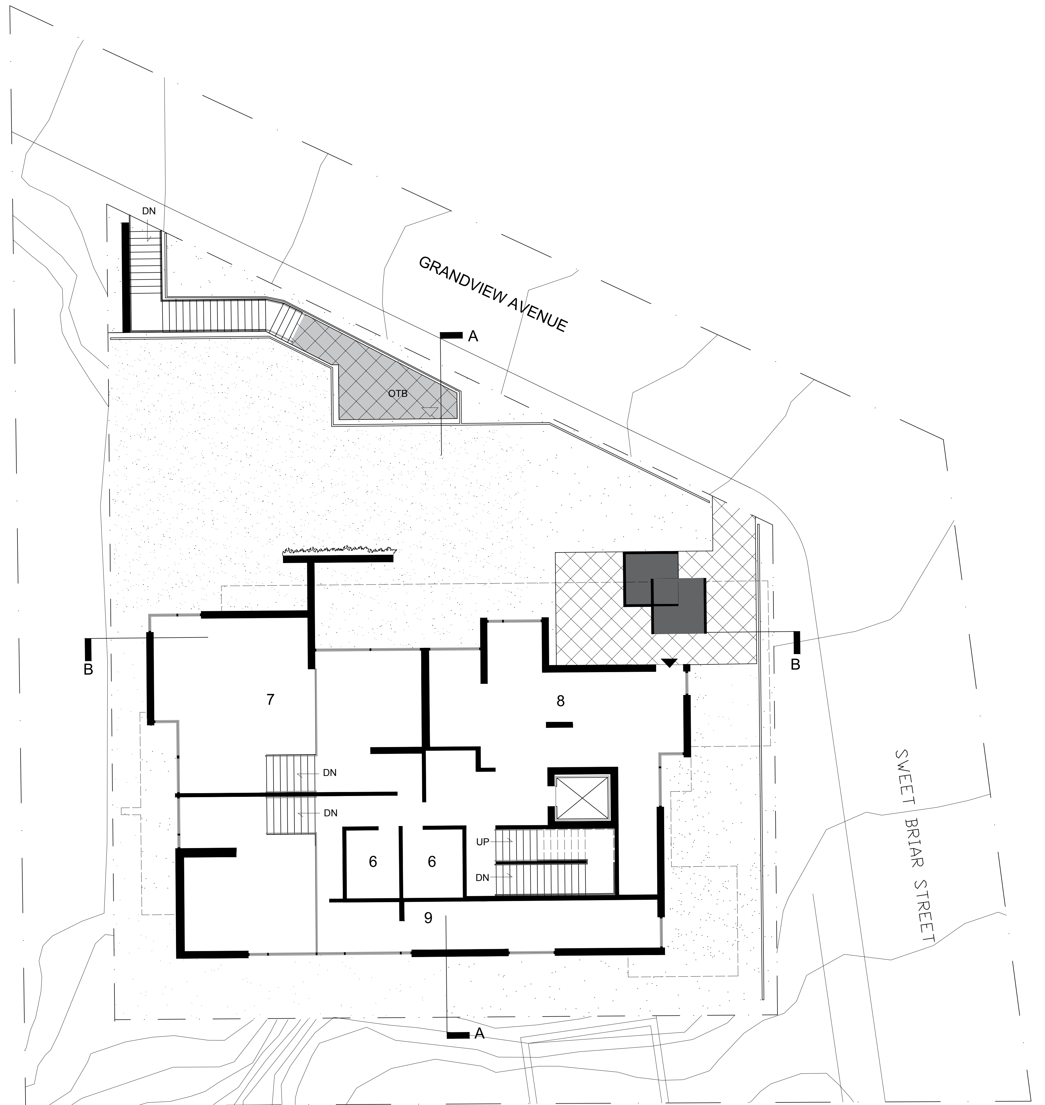
SITE/FLOOR 1 PLAN SCALE = 1'-0" = \frac{1}{8} "
