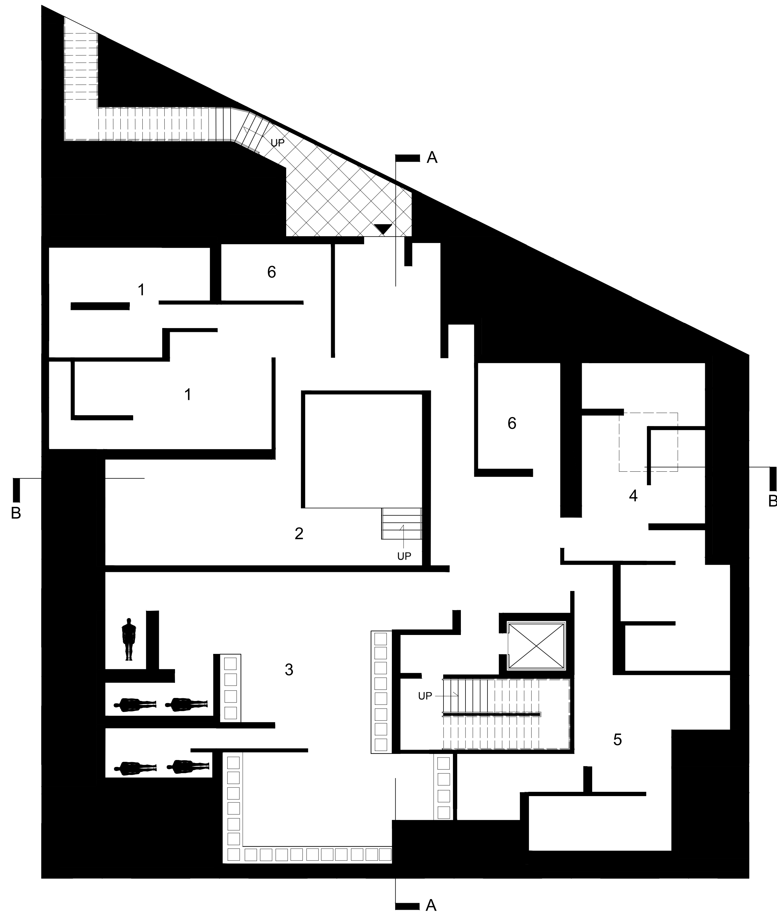
BASEMENT PLAN SCALE = 1'-0" = \frac{1}{8} "
